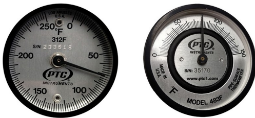
PTC® Surface Thermometers
